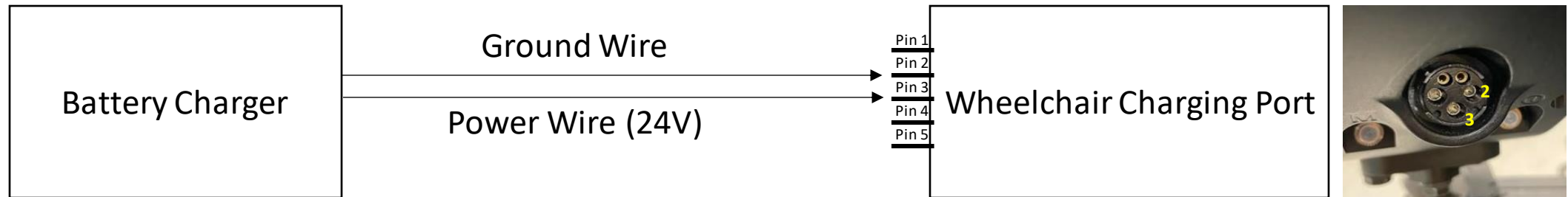
Figure: Wheelchair Charger Wiring Diagram
