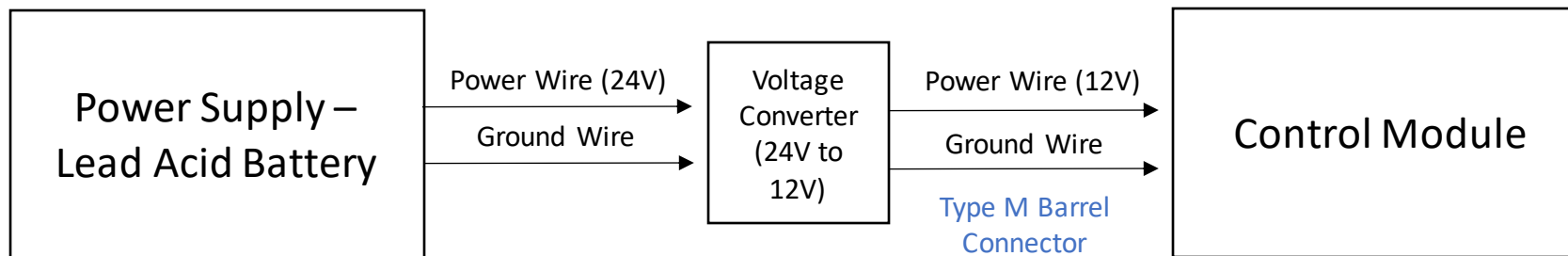
Figure: Control Module Power Wiring Diagram
