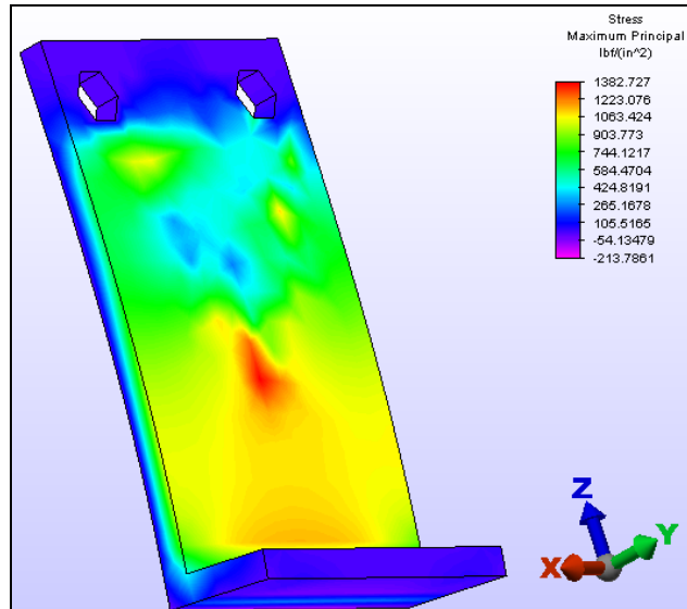
Maximum Principal Stress of Support Option 3 (in psi)
