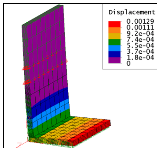
Maximum Displacement of Support Option 2 (in inches)
