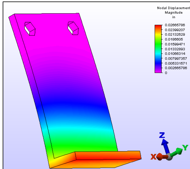
Maximum Displacement of Support Option 3 (in inches)
