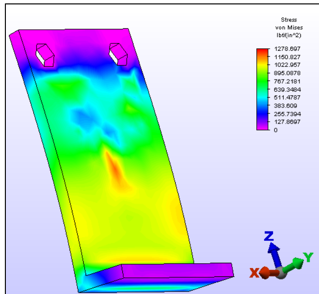
von Mises Stress of Support Option 3 (in psi)
