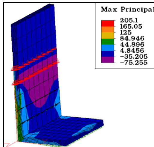
Maximum Principal Stress of Support Option 2 (in psi)
