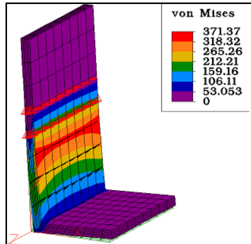
von Mises Stress of Support Option 2 (in psi)
