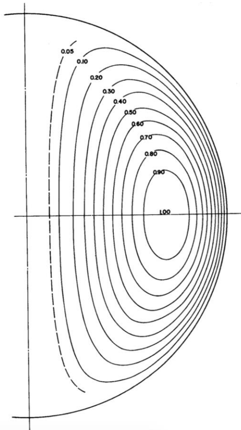
Figure d1. Flow regime within a sphere for the proof of concept of bulb mixing.
