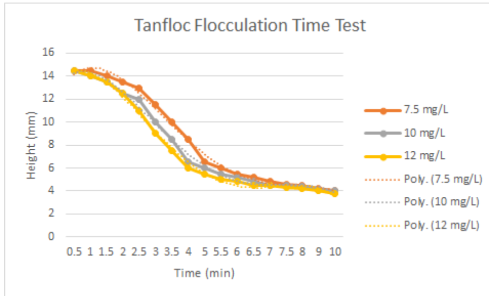
Figure a1. Experimental Tanfloc sedimentation data.
