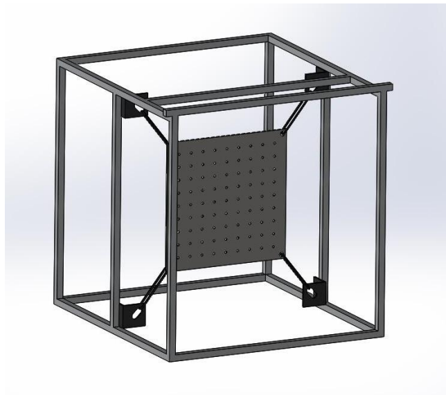
Figure 7: General concept for decoupling fixture plate via suspension
