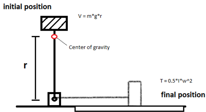
Figure 8: Sketch of the initial and final states of the hammer in the new configuration
