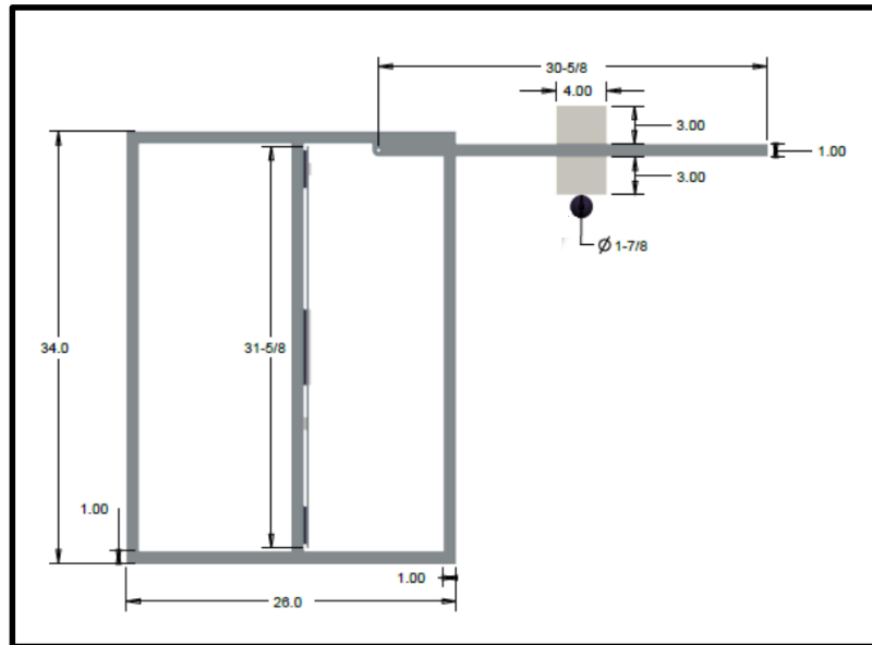
Figure 4. Side view of Last Year's Rig [inches]
