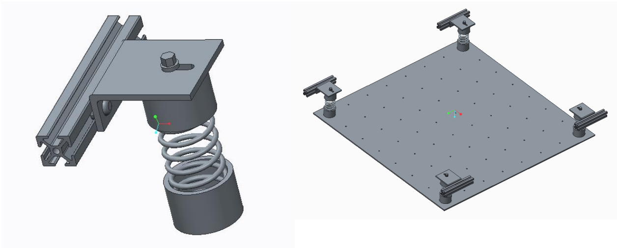
Figure 6: General concept for spring isolators (left), and all four attached to fixture plate (right)
