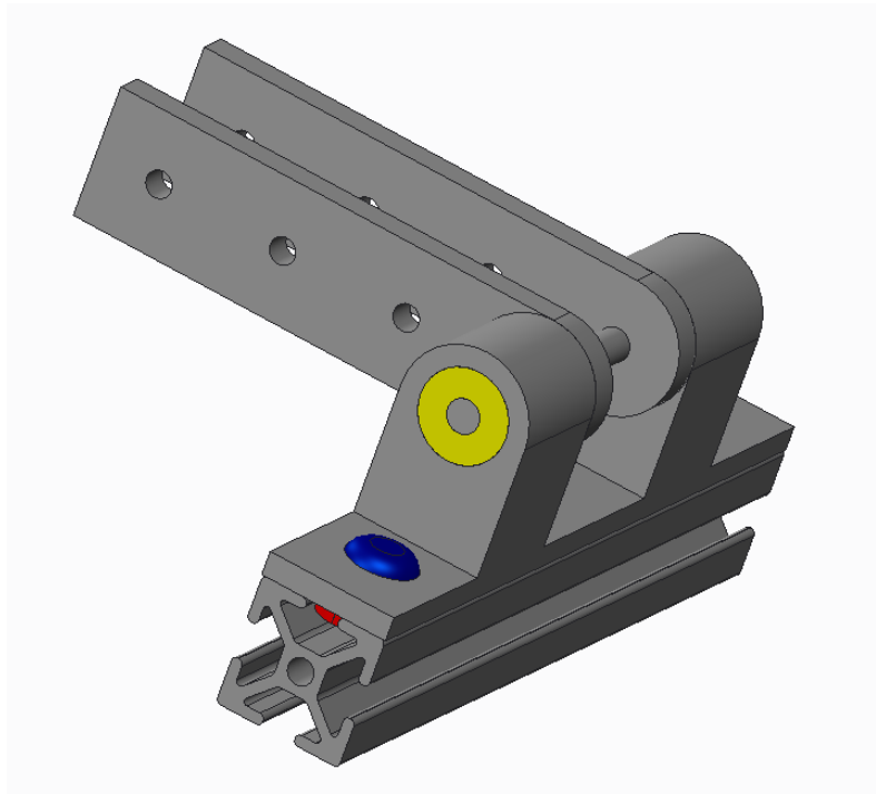
Figure 5: Proposed design for hammer's pivot mechanism
