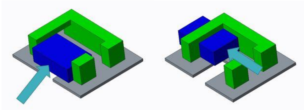
Figure 8: Dimension check process for 2 nd gauge block design
