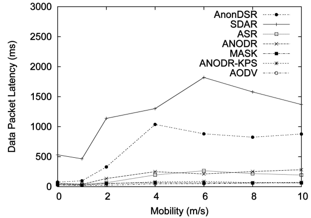
Fig. 6. Data packet latency (ms).
