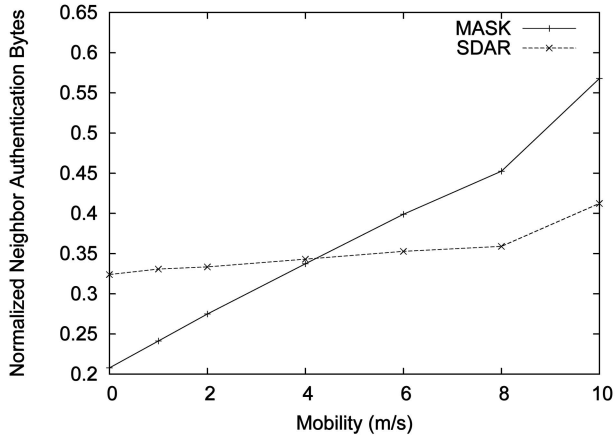
Fig. 8. Normalized neighbor authentication bytes.
