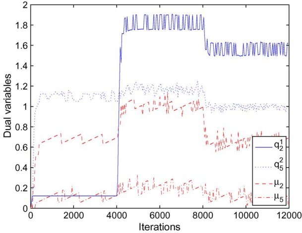
Fig. 5. Dual variables produced by the distributed algorithm. \alpha = 0.1 .
