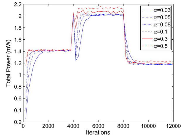
Fig. 3. Power consumption from distributed algorithm as the value of \alpha varies from 0.03 to 0.5.
