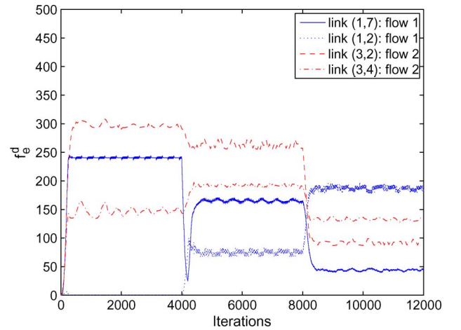
Fig. 8. Average data rates ( f_e^d ) for different flows on four links, \alpha = 0.1 .
