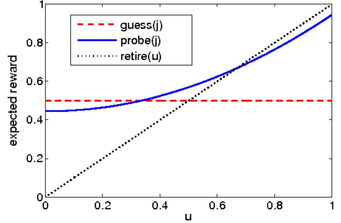
Fig. 1. As described in Section III-A, when j is the only unprobed channel and X_j is uniformly distributed in [0, 1] , the expected reward from actions \text{guess}(j) , \text{probe}(j) , and \text{retire}(u) as functions of u . Note that a_j = 2/3 (the crossing point of solid and dotted lines) and b_j = 1/3 (the crossing point of solid and dashed lines).
