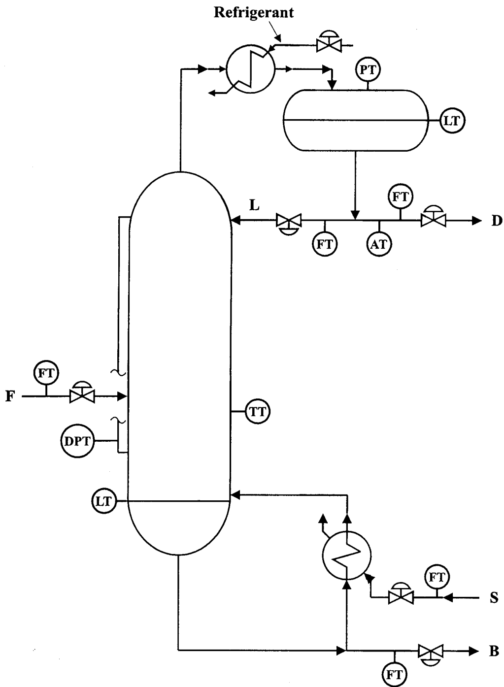
Figure 1 Schematic of a C 2 splitter with the sensors and control valves.
