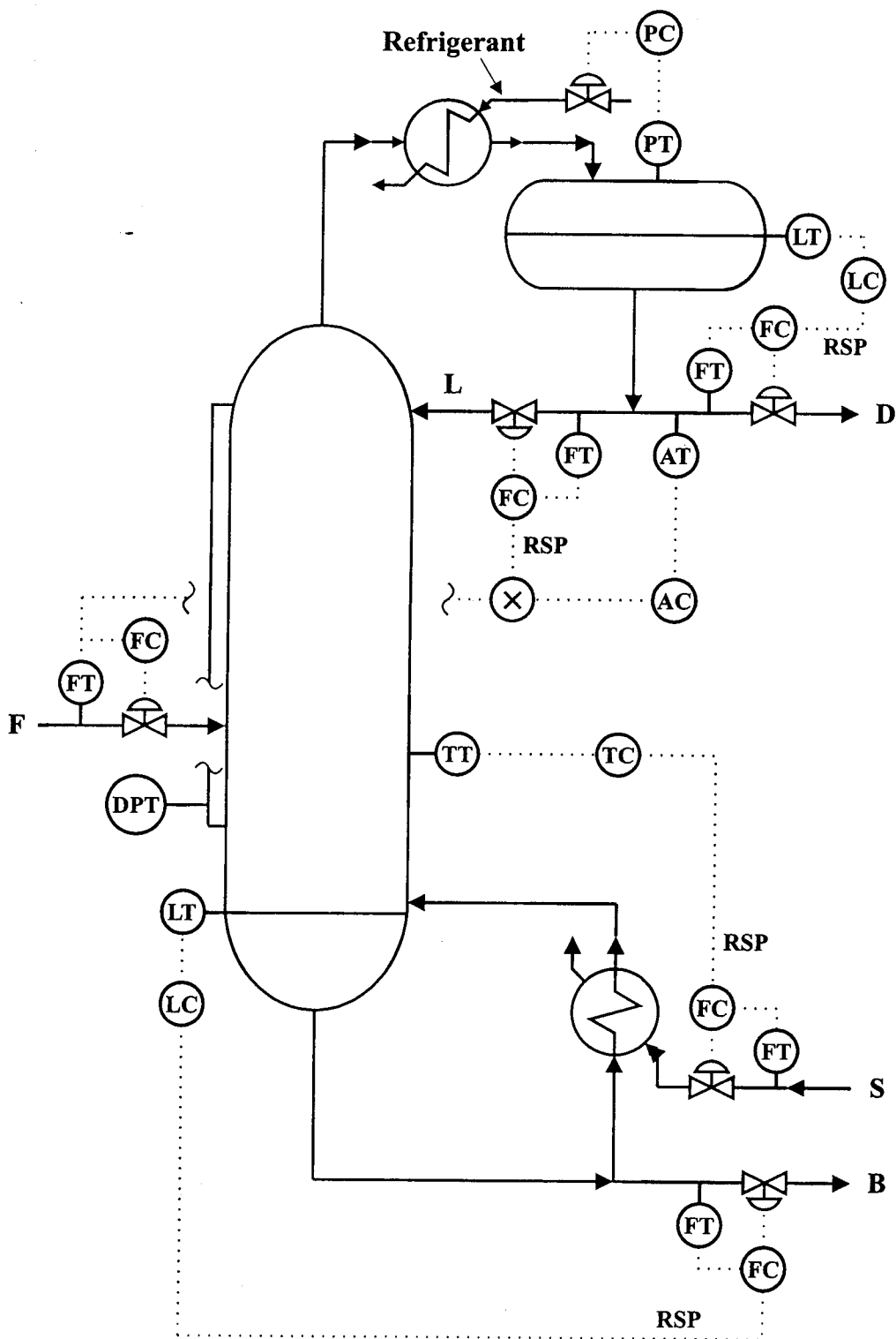
Figure 2 Schematic of a C_2 splitter with the (L,V) configuration applied.
