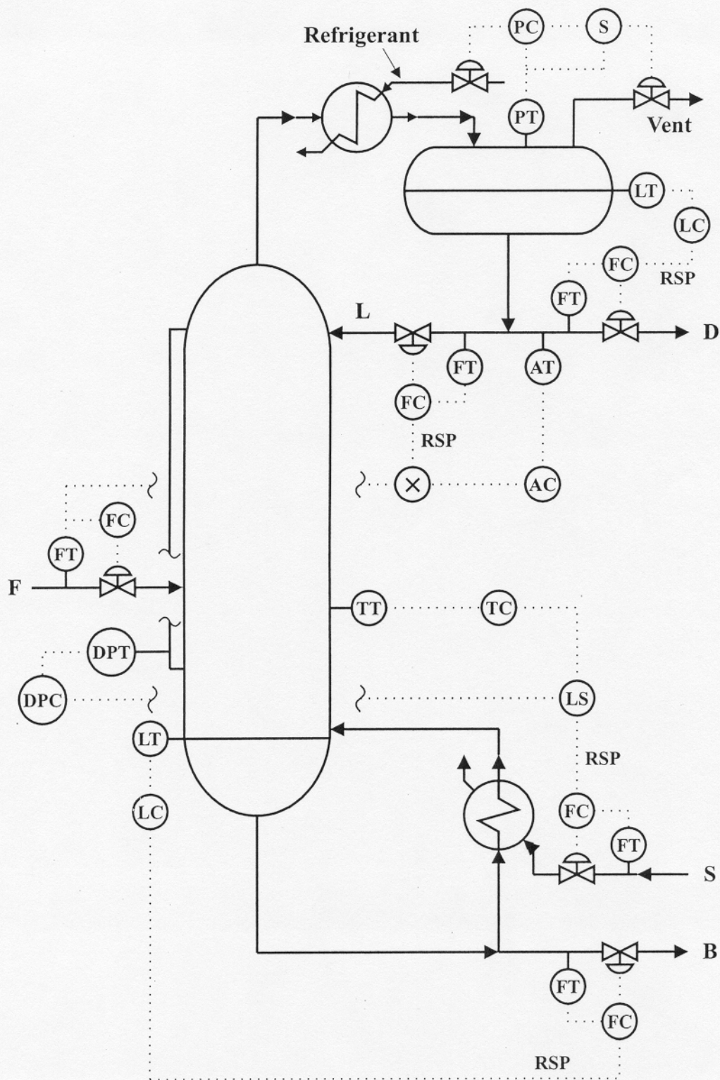
Figure 3 Schematic for a C 2 splitter with complete control configuration.
