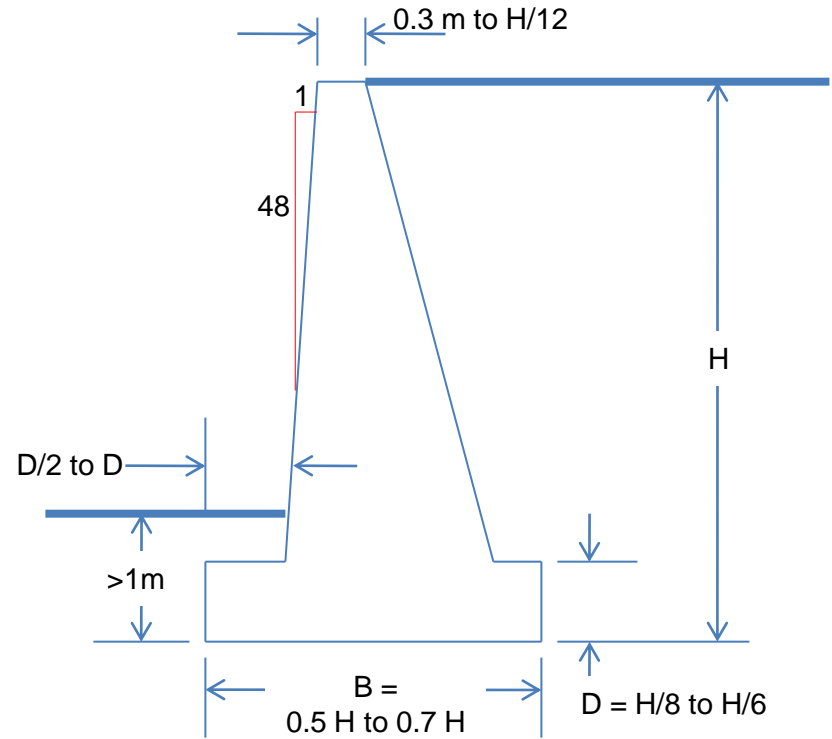
Gravity Retaining Wall
