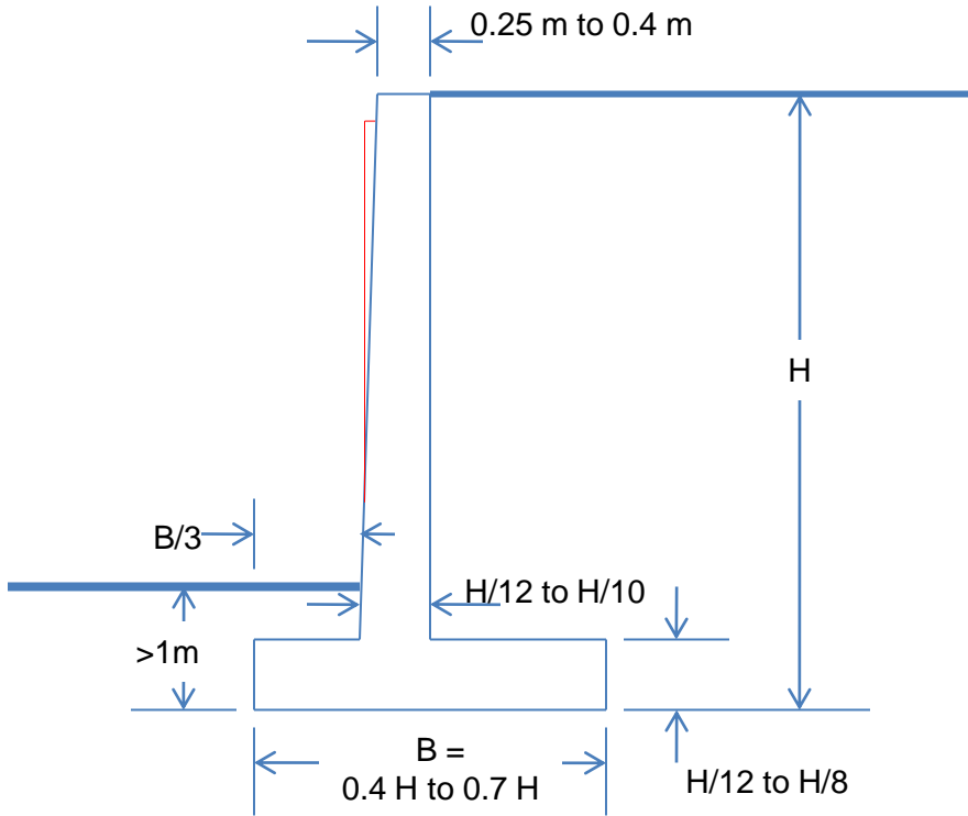
Cantilever Retaining Wall
